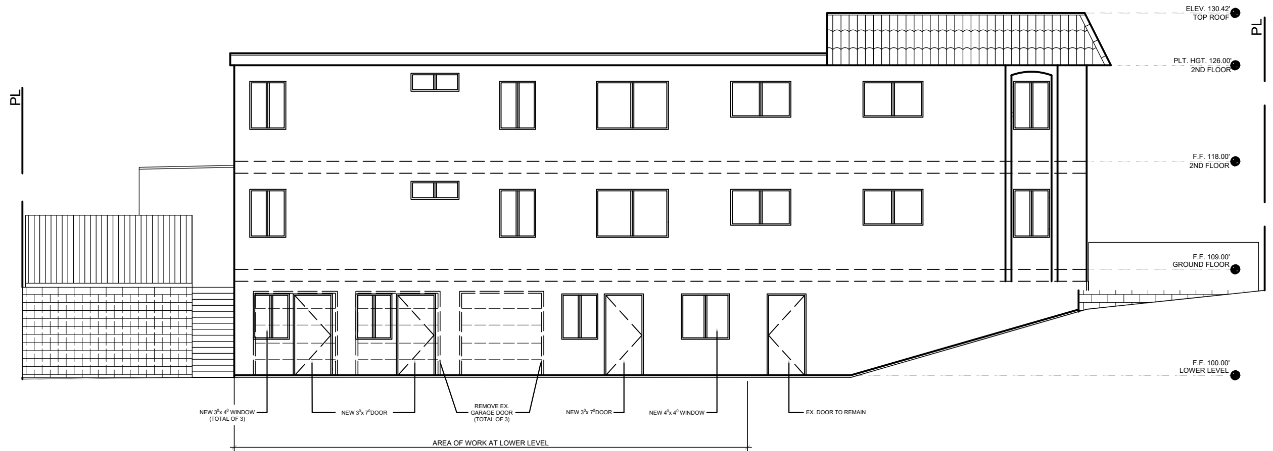
SOUTH EXTERIOR ELEVATION (FOR REFERENCE ONLY)
